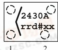
Flip Chip, Top View with Laser Mark, Contacts Not Visible. “rrd” = Revision/Date #xx = Lot Number See 56-G7016-001 for package outline.
