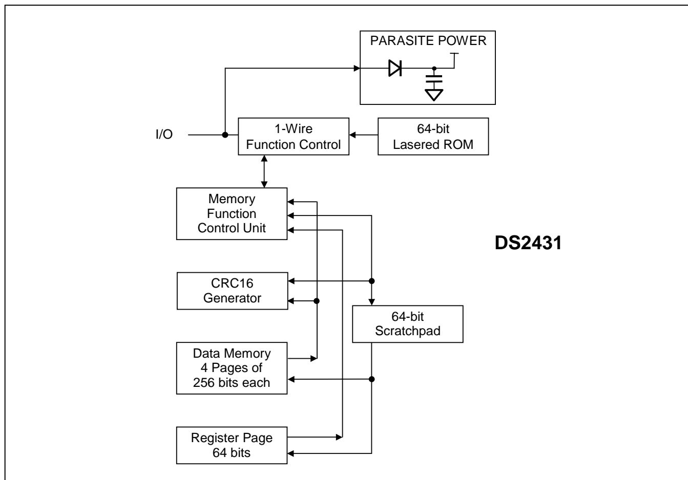
Figure 1. Block Diagram
