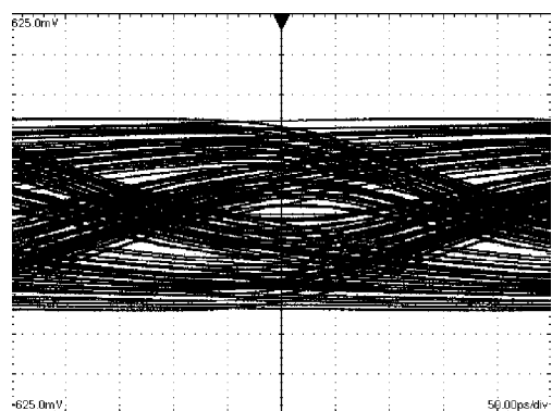
A 3.125 Gbps NRZ PRBS-7 After 40" Differential FR-4 Stripline V:125 mV / DIV, H:50 ps / DIV
