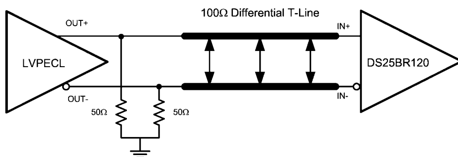
Typical LVPECL Driver DC-Coupled Interface to DS25BR120 Input
