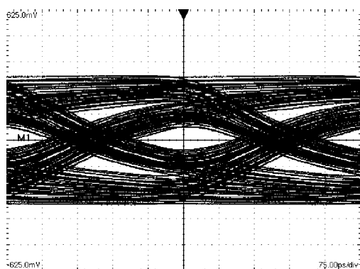
A 2.5 Gbps NRZ PRBS-7 After 40" Differential FR-4 Stripline V:125 mV / DIV, H:75 ps / DIV
