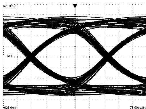
An Equalized (with PE) 2.5 Gbps NRZ PRBS-7 After 40" Differential FR-4 Stripline V:125 mV / DIV, H:75 ps / DIV
