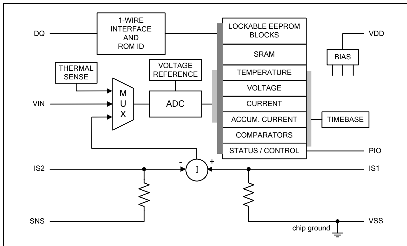
Figure 2. FUNCTIONAL DIAGRAM
