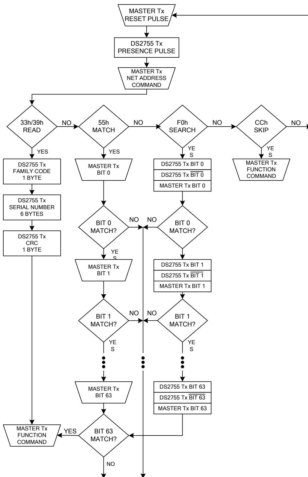
Figure 17. NET ADDRESS COMMAND FLOW CHART
