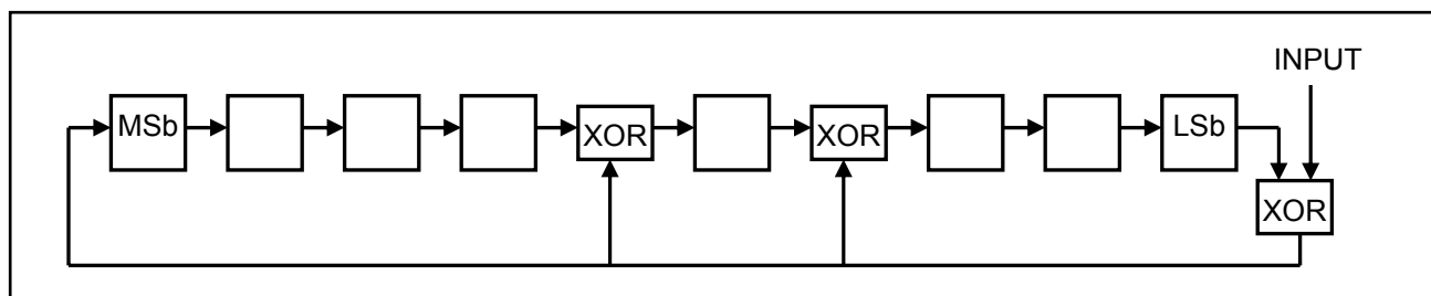
Figure 15. 1-WIRE CRC GENERATION BLOCK DIAGRAM
