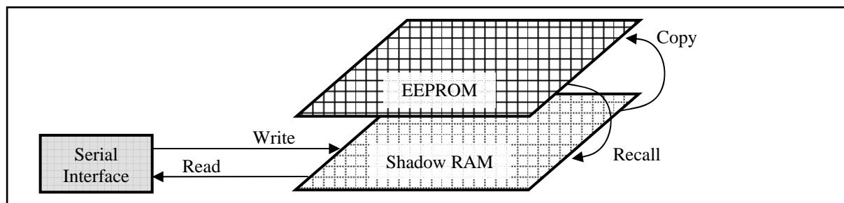
Figure 9. EEPROM Access via Shadow RAM
