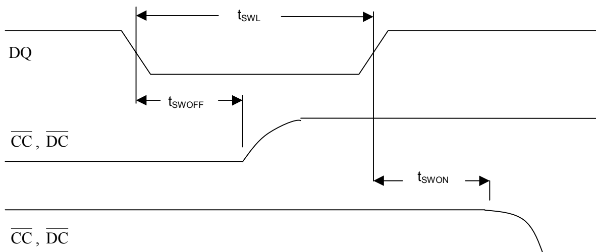
Figure 19. SWAP COMMAND TIMING
