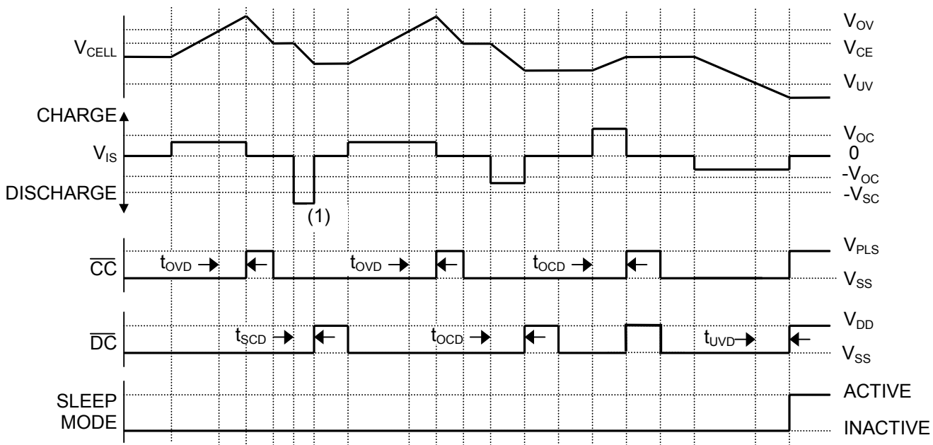
Figure 3. Li+ PROTECTION CIRCUITRY EXAMPLE WAVEFORMS
