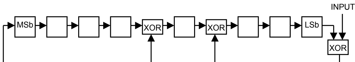
Figure 14. 1-WIRE CRC GENERATION BLOCK DIAGRAM
