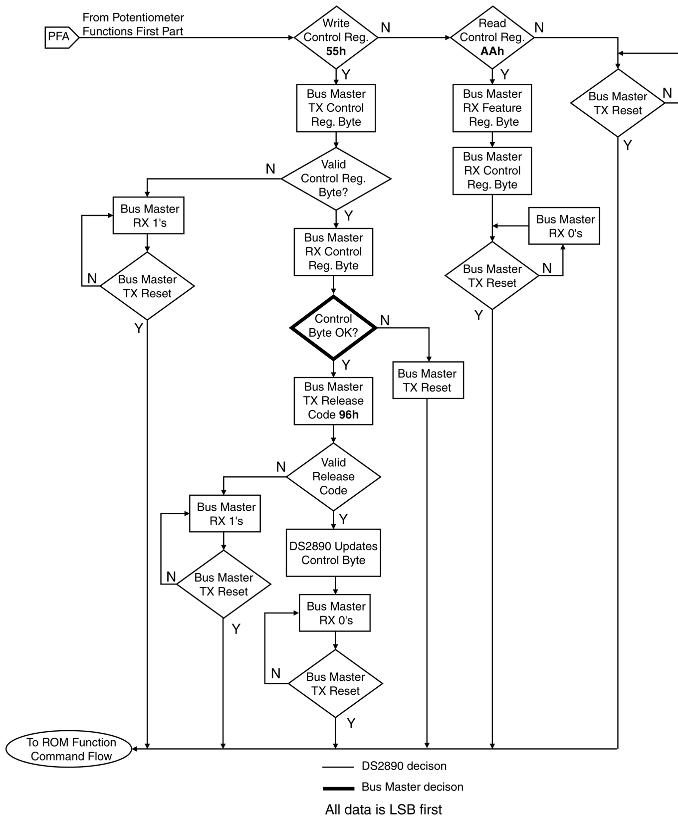
Figure 17. POTENTIOMETER FUNCTION COMMAND FLOW (continued)
