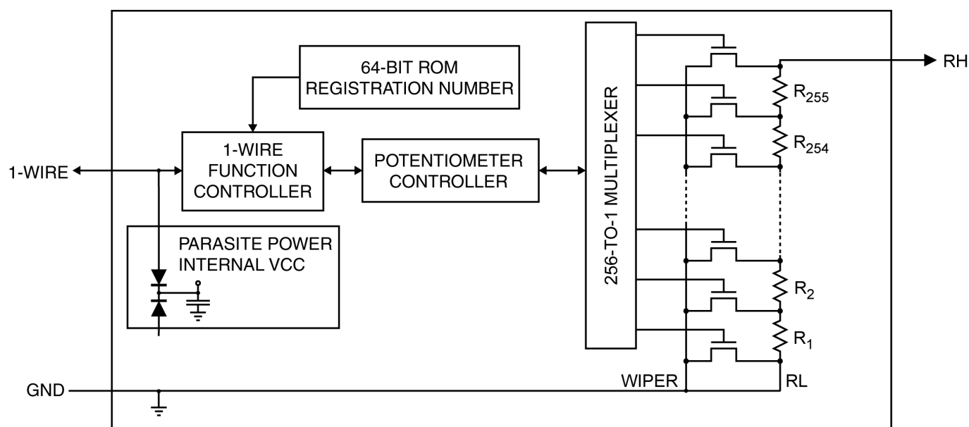
Figure 9. DS2890 TO-92 CONFIGURATION BLOCK DIAGRAM
