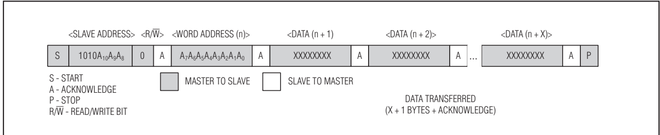
Figure 5. Data Write—DS32B35 FRAM Slave Receiver Mode
