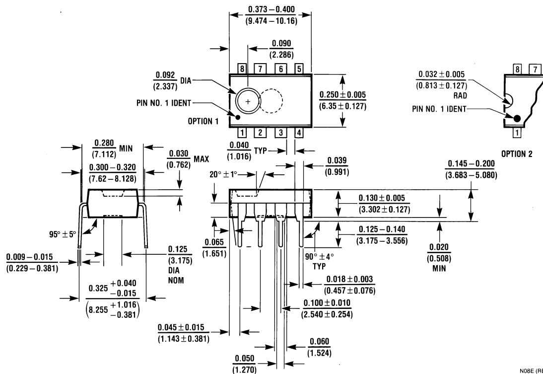
8-Lead Molded Dual-In-Line Package (N) Order Number DS36277TN NS Package Number N08E
