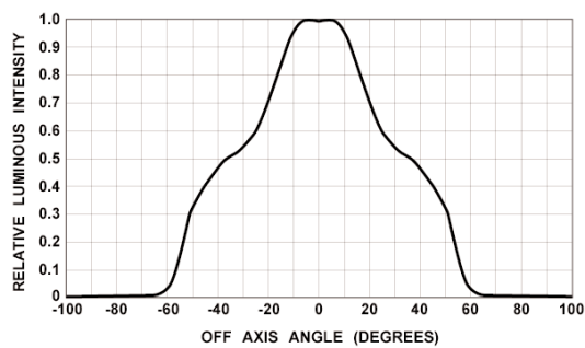
Figure 5c. HPWT-Mx02 Relative Luminous Intensity vs. Off Axis Angle.
