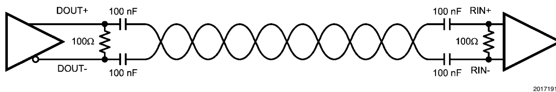
FIGURE 17. AC Coupled Application
