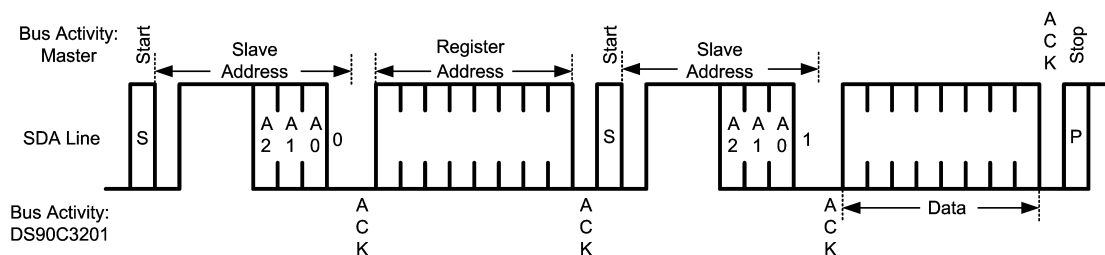
FIGURE 14. Byte Read
