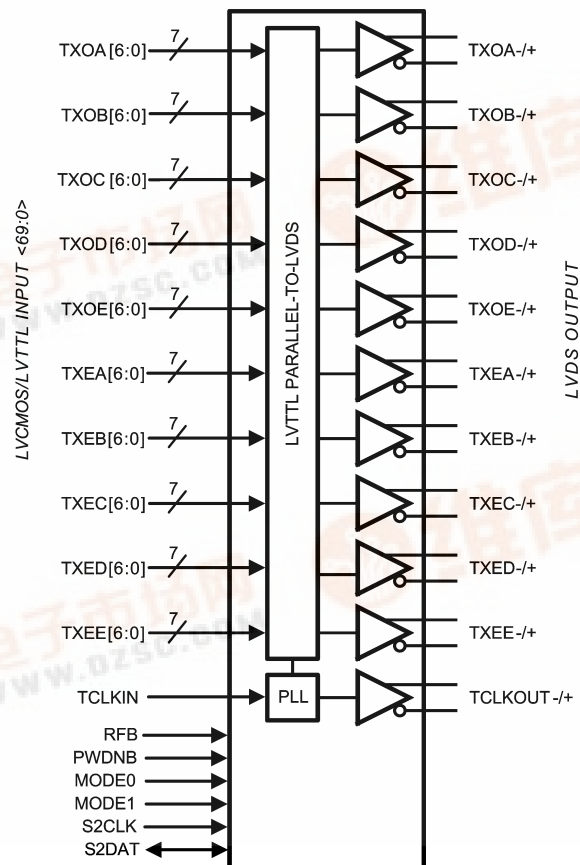
FIGURE 1. Transmitter Block Diagram
