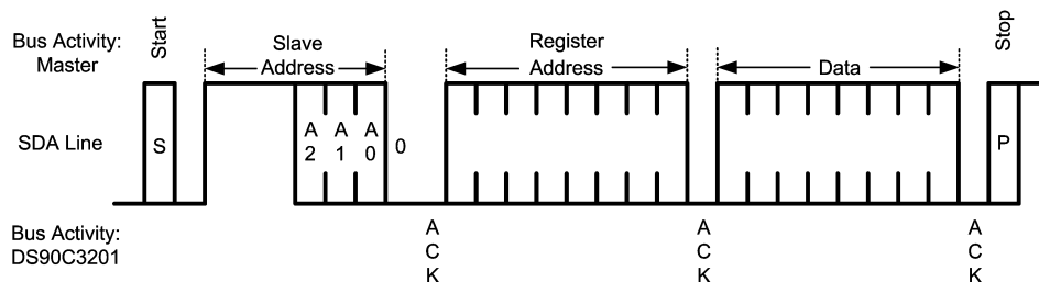
FIGURE 15. Byte Write
