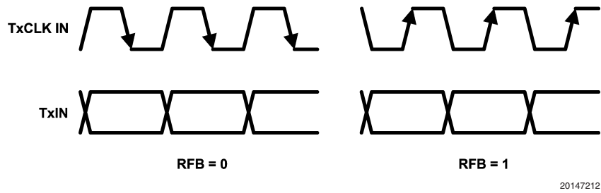
FIGURE 10. LVTTLL Input Programmable Strobe Select
