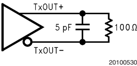
FIGURE 3. DS90C365A (Transmitter) LVDS Output Load. 5pF is showed as board loading
