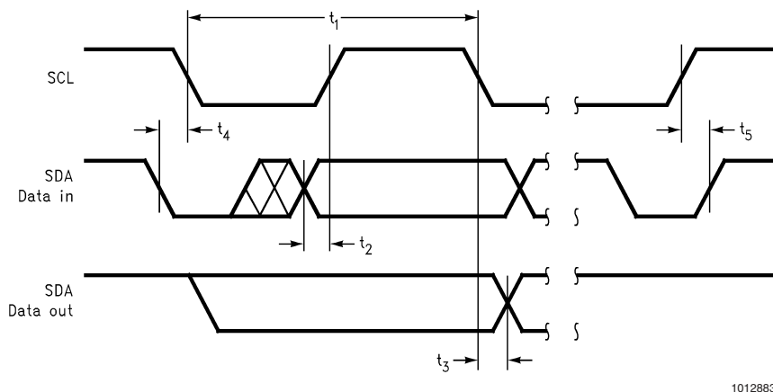
FIGURE 1. Two-Wire Serial Communication Interface Timing Diagram when I2CSEL = Vcc
