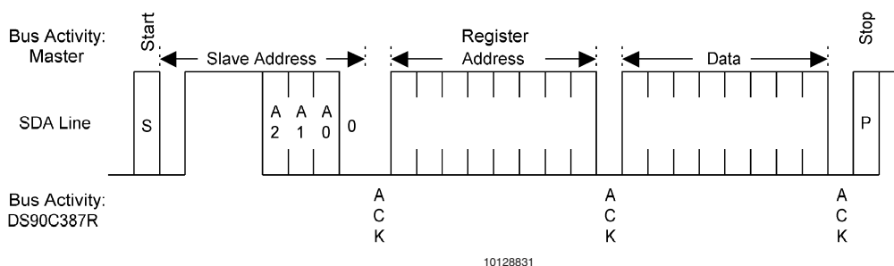
FIGURE 15. Byte Write
