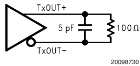
FIGURE 3. DS90CF363B (Transmitter) LVDS Output Load
