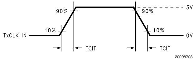
FIGURE 5. DS90CF363B (Transmitter) Input Clock Transition Time
