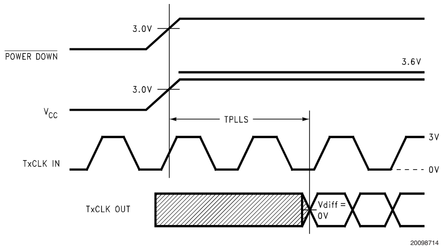
FIGURE 8. DS90CF363B (Transmitter) Phase Lock Loop Set Time
