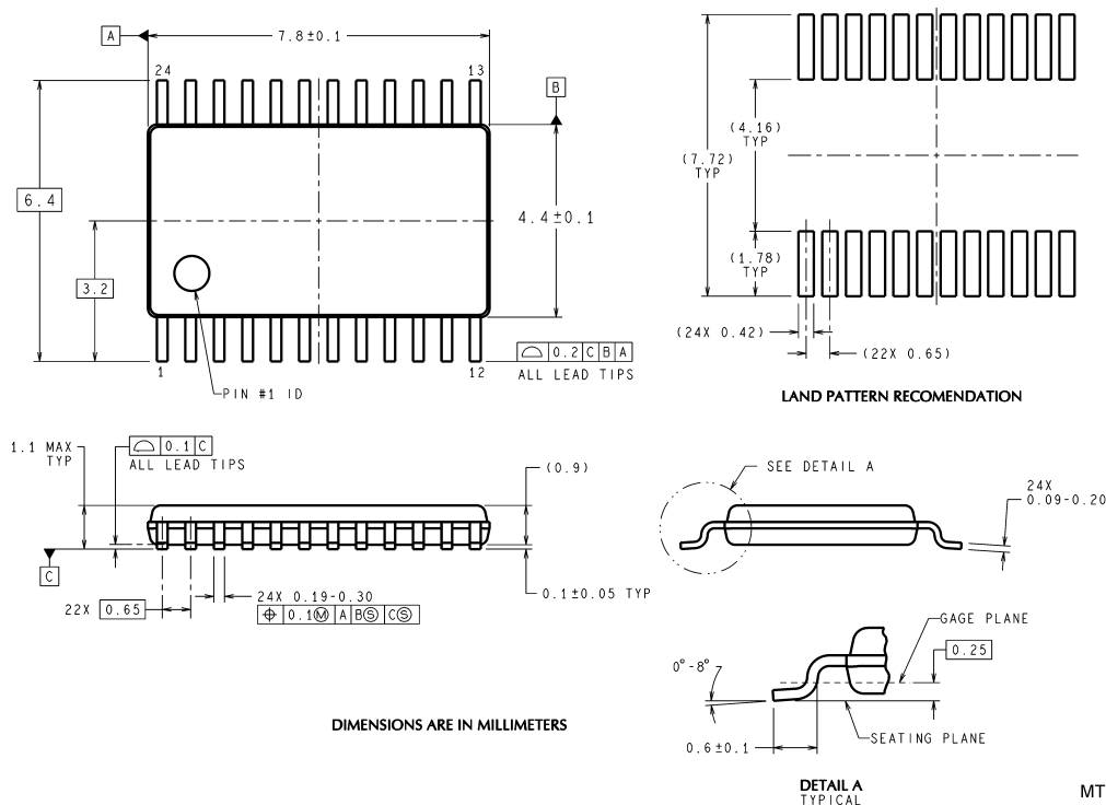
24-Pin TSSOP Package Drawing Dimensions shown in millimeters Order Number DS92CK16TMT NS Package Number MTC24
