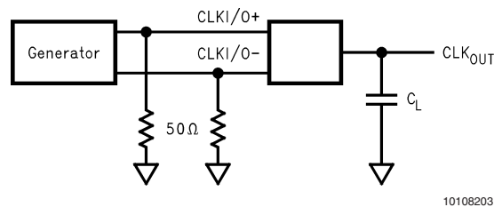
FIGURE 1. Receiver Propagation Delay and Transition Time Test Circuit
