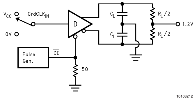
FIGURE 10. Driver TRI-STATE Test Circuit
