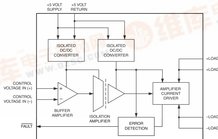
Figure 1. Simplified Schematic
