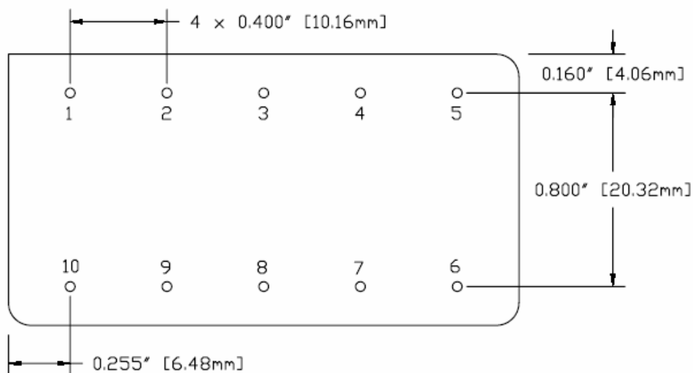
BOTTOM VIEW
