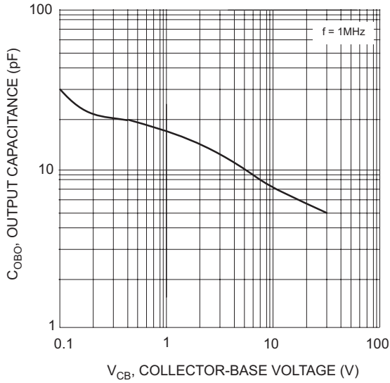
V_{CB} , COLLECTOR-BASE VOLTAGE (V) Fig. 3, Output Capacitance vs. Collector-Base Voltage (NPN Transistor)
