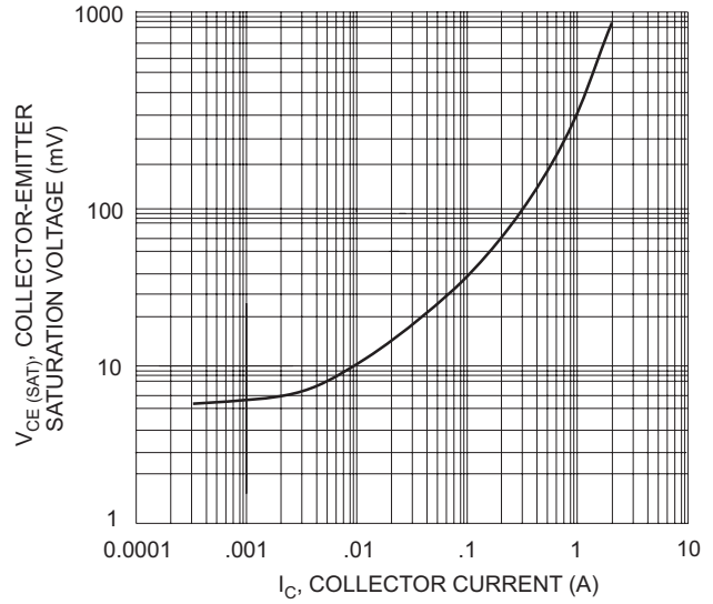
I_C , COLLECTOR CURRENT (A) Fig. 4, Collector Saturation Voltage vs Collector Current (NPN Transistor)
