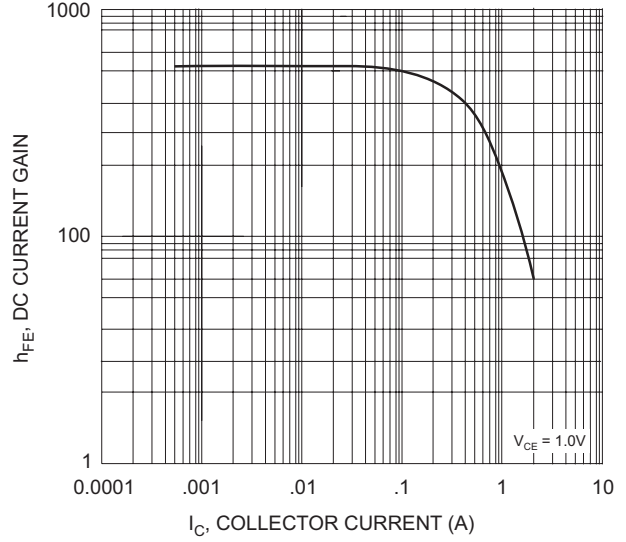
I_C , COLLECTOR CURRENT (A) Fig. 2, Typical DC Current Gain vs Collector Current (NPN Transistor)
