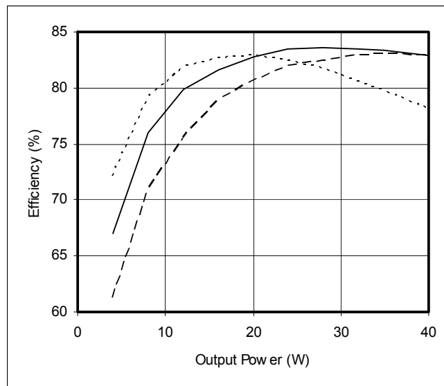
Figure 8 – DVTR2812D Efficiency (%) vs. Output Power (W)
