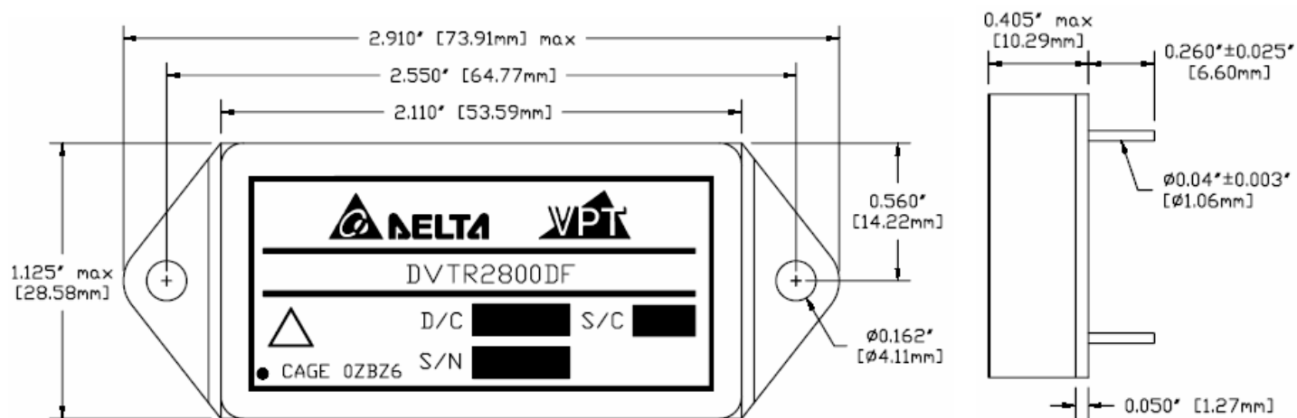
TOP VIEW
