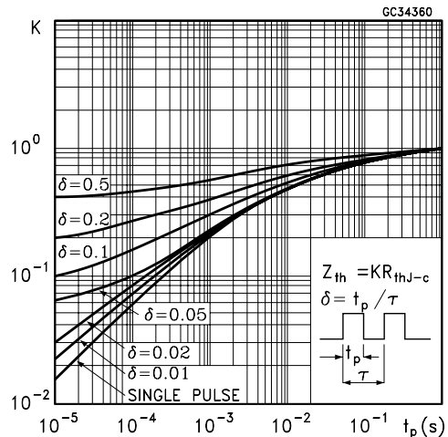
Figure 7: Thermal Impedance For DPAK/IPAK
