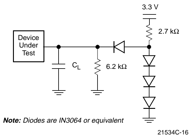
Figure 11. Test Setup
