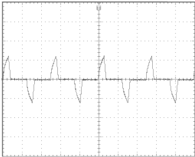
Figure 6: LF Input Duty Cycle = +75%
