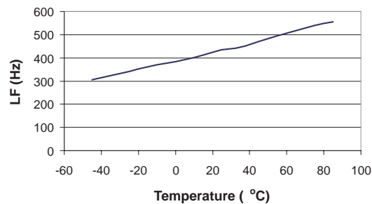
Output Frequency vs. Ambient Temperature
