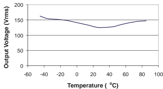
Output Voltage (Vrms) vs. Ambient Temperature
