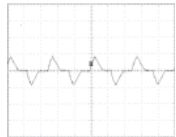
Figure 6: LF Input Duty Cycle = +75%
