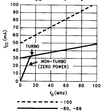
85C220/85C224 I CC vs Frequency
