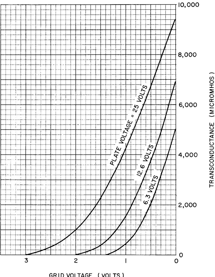
TRANSCONDUCTANCE CHARACTERISTICS
