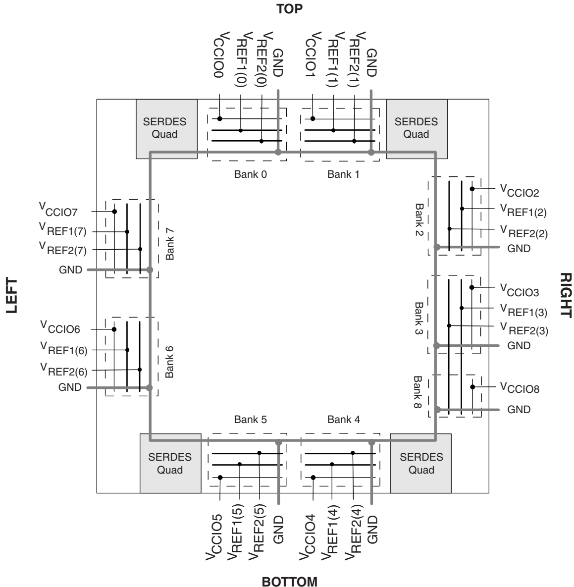
Figure 2-38. LatticeECP2M Banks
