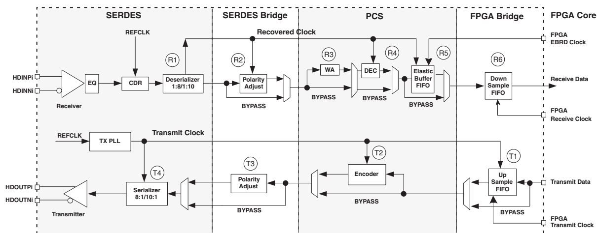
Figure 3-12. Transmitter and Receiver Block Diagram
