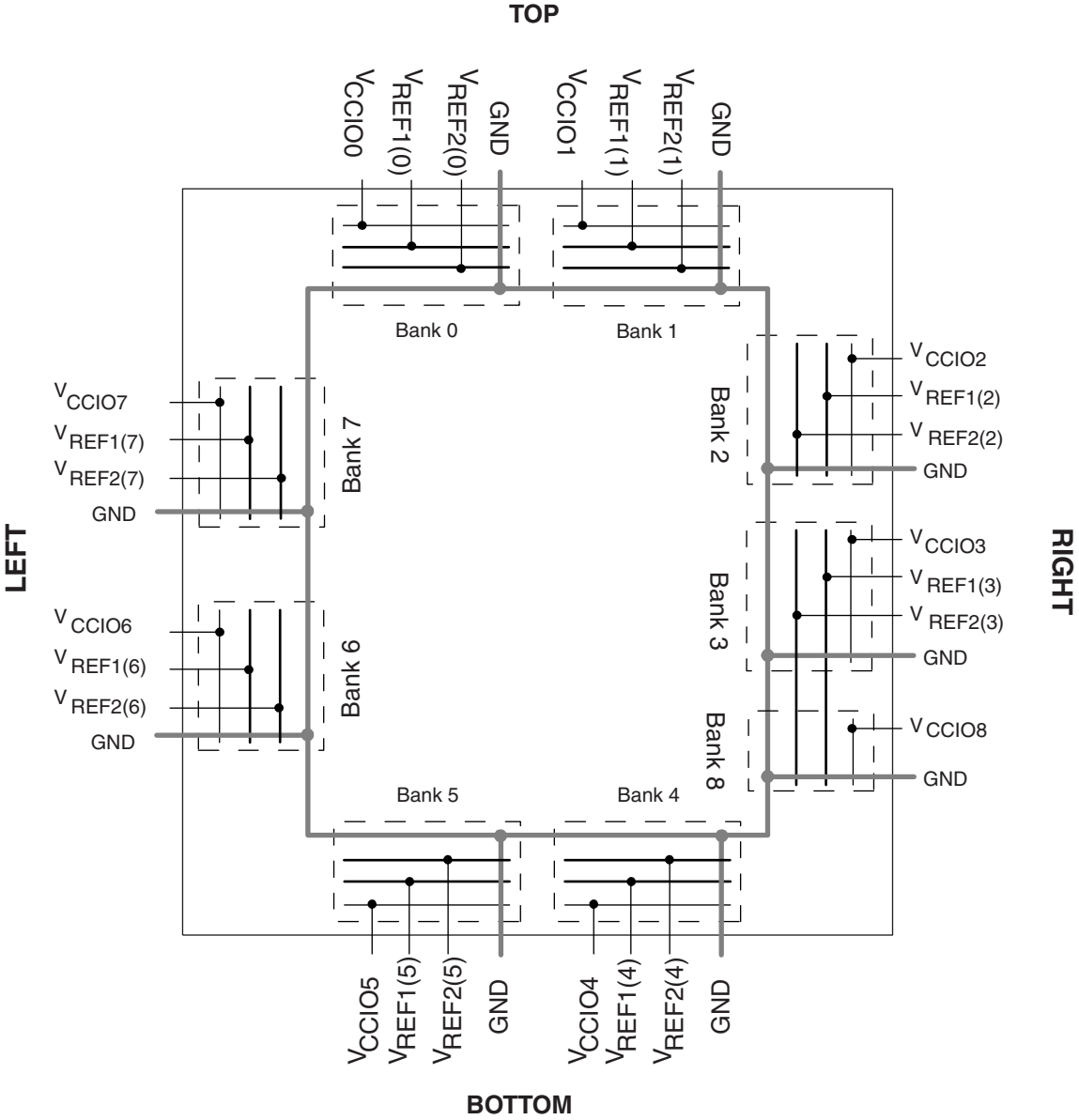
Figure 2-37. LatticeECP2 Banks
