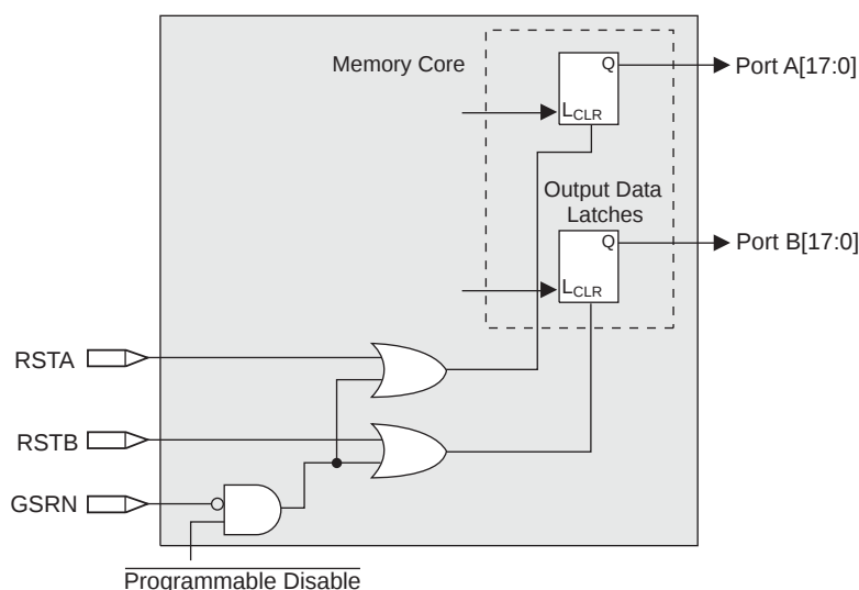
Figure 2-20. Memory Core Reset
