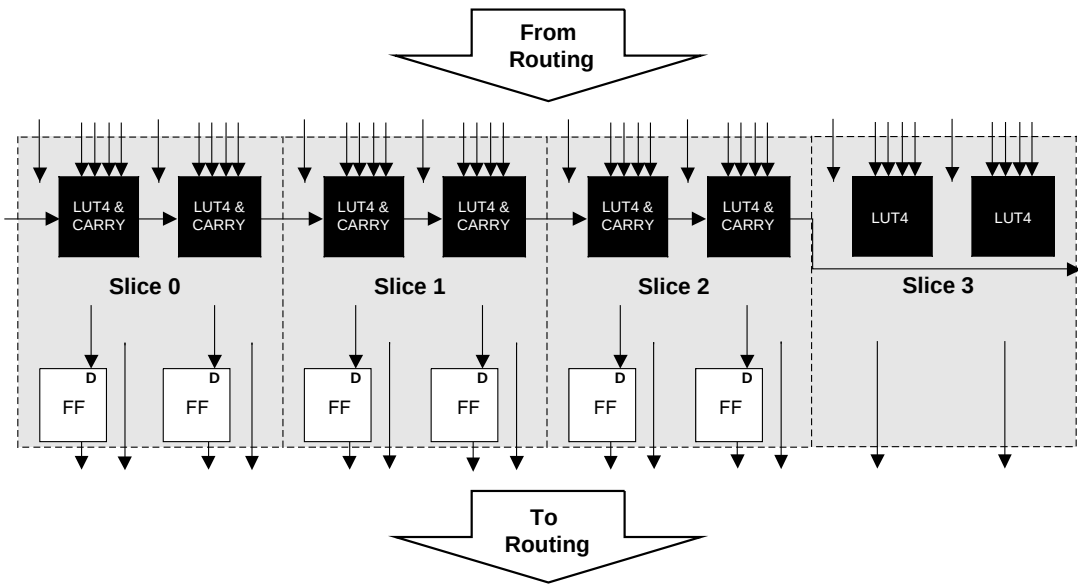
Figure 2-3. PFU Diagram
