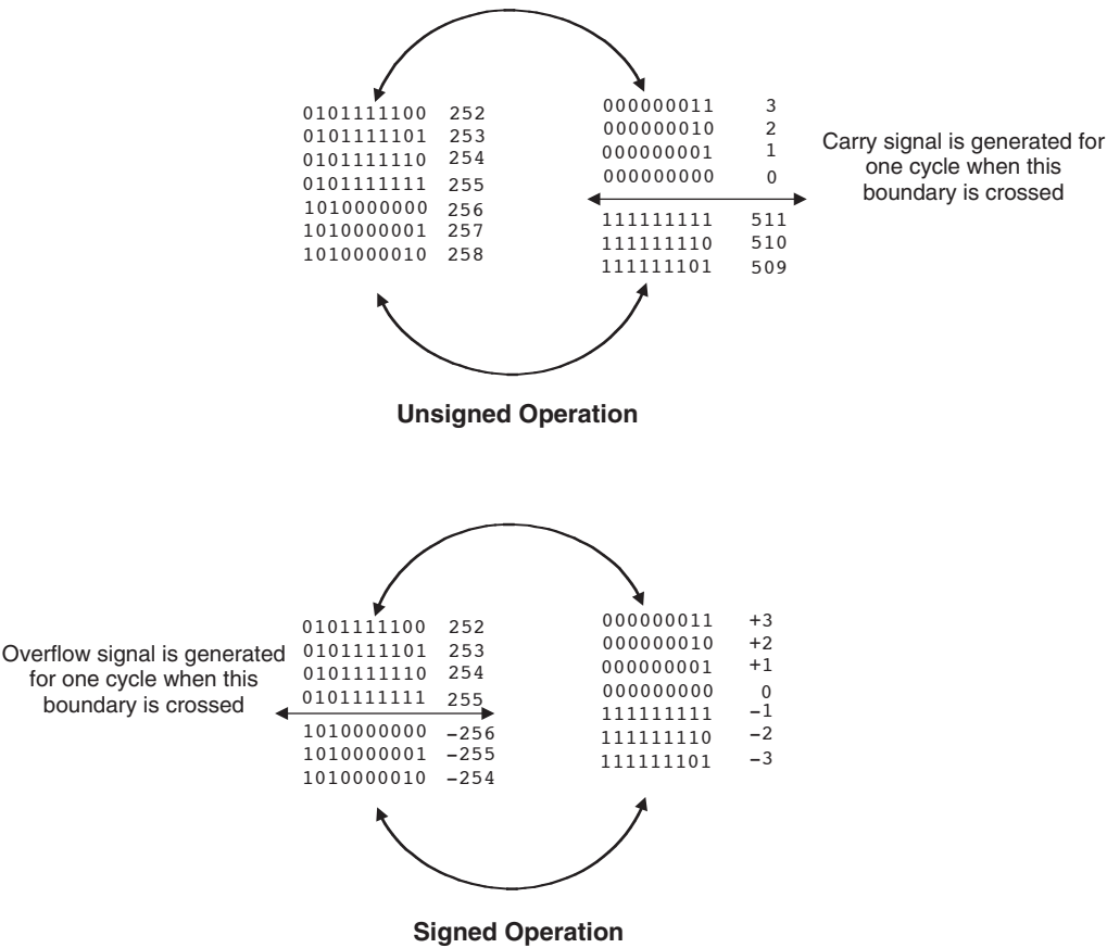
Figure 2-27. Accumulator Overflow/Underflow
