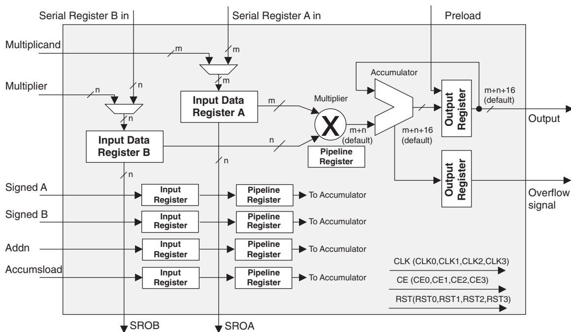
Figure 2-24. MAC sysDSP
