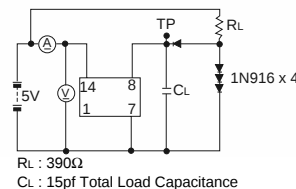
Figure 3) Measurement Circuit (includes probe capacitance)
