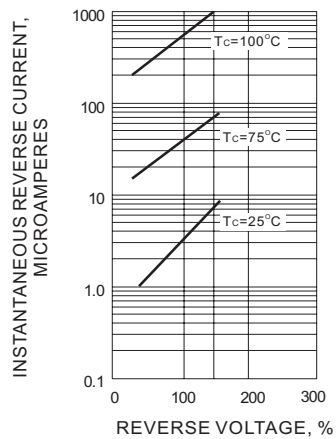
Fig.3-TYPICAL REVERSE CHARACTERISTICS
