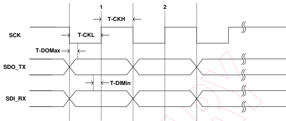
Fig. 5-7 Timing diagram for SPI master mode
