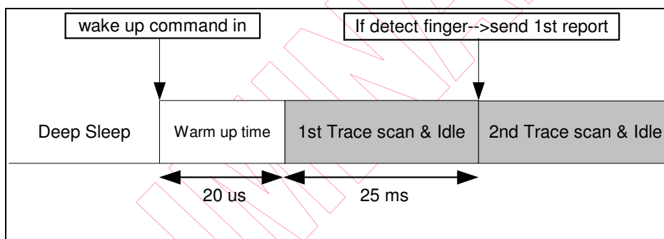
Fig. 7-2 Wake-up Timing from Deep Sleep Mode
