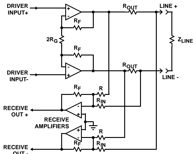
FIGURE 43. TYPICAL LINE INTERFACE CONNECTION
