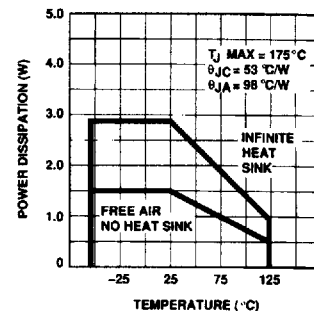
20-Lead LCC Maximum Power Dissipation vs Ambient Temperature
