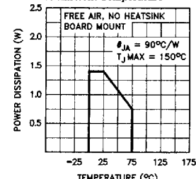
18-Lead SOI Maximum Power Dissipation vs Ambient Temperature
