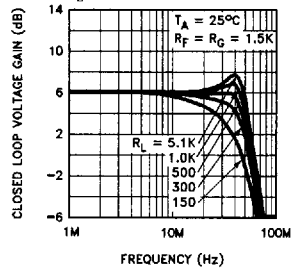
Voltage Gain vs Frequency A_V = +2 V_S = \pm 5V
