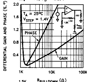
Differential Gain and Phase vs RL A_V = +2, V_S = \pm 5V
