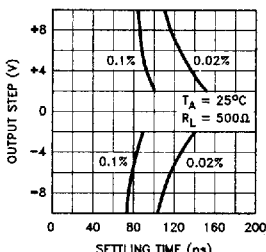
Settling Time vs Output Swing A_V = +1, V_S = \pm 15V
