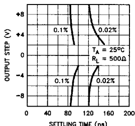
Settling Time vs Output Swing A_V = +10, V_S = \pm 15V
