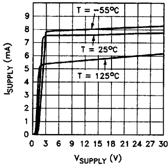
Supply Current vs Supply Voltage— Both Amplifiers
