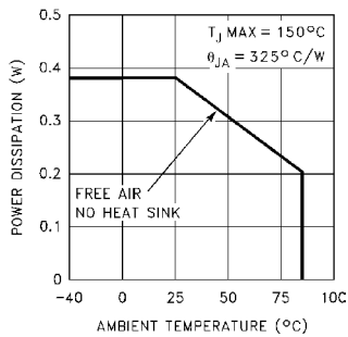
5-Pin Plastic SOT-23 Maximum Power Dissipation vs Ambient Temperature
