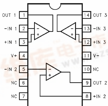
EL2344 14-PIN PDIP, SO TOP VIEW
