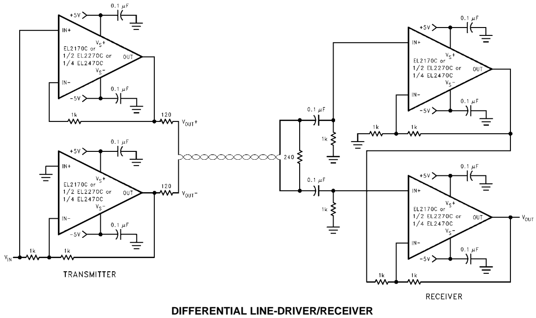
DIFFERENTIAL LINE-DRIVER/RECEIVER
