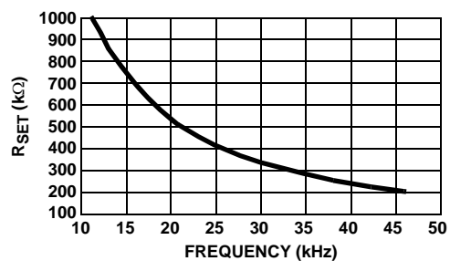
FIGURE 1. R SET vs HORIZONTAL FREQUENCY
