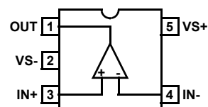
EL5101 (5 LD SOT-23) TOP VIEW
