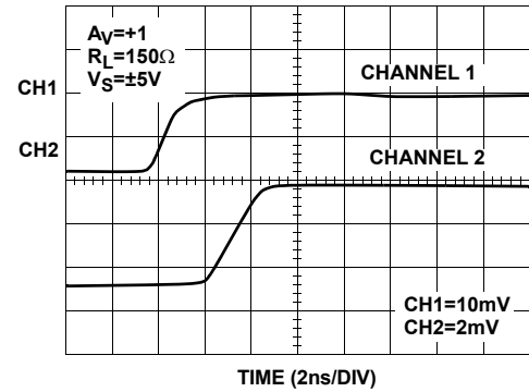
FIGURE 18. SMALL SIGNAL RISE TIME
