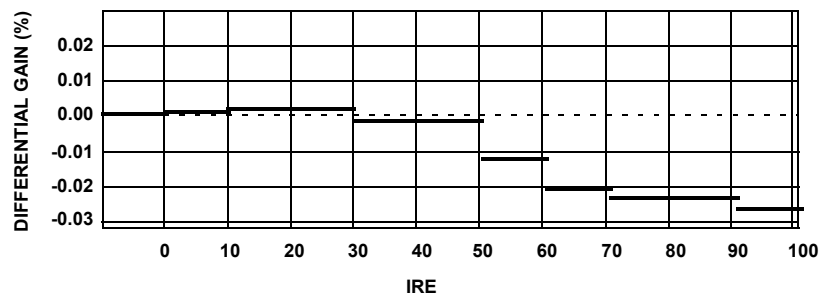
FIGURE 27. DIFFERENTIAL GAIN (%)
