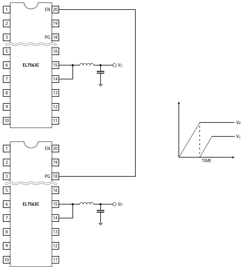
Figure 4. Offset Tracking
