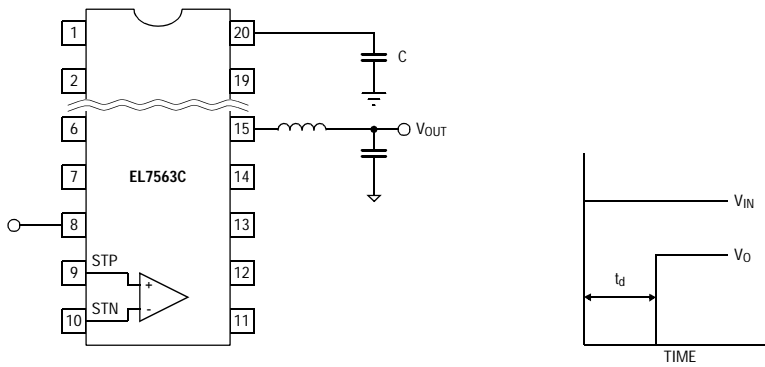
Figure 6. Start-up Delay
