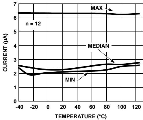
FIGURE 16. SUPPLY CURRENT vs TEMPERATURE V_S = \pm 2.5V DISABLED. R_L = INF
