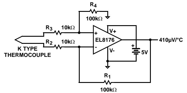
FIGURE 42. THERMOCOUPLE AMPLIFIER
