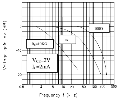
Fig.11 Frequency Response
