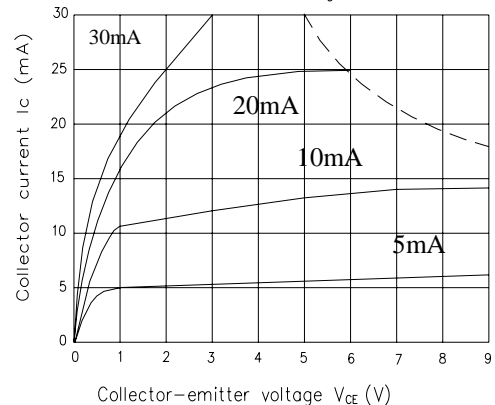
Fig.6 Collector Current vs. Collector-emitter Voltage (Ta=25°C)
