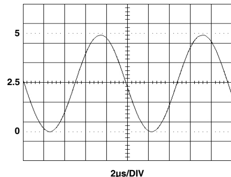
FIGURE 24. OUTPUT SWING
