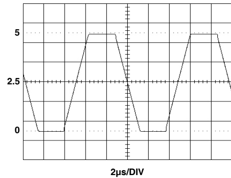
FIGURE 22. OUTPUT SWING
