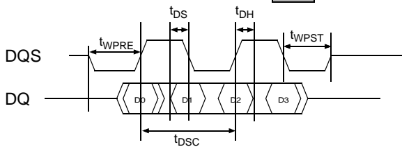
WRITE Operation
