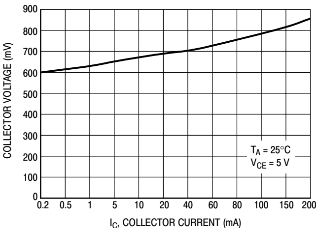
Figure 9. On Voltage
