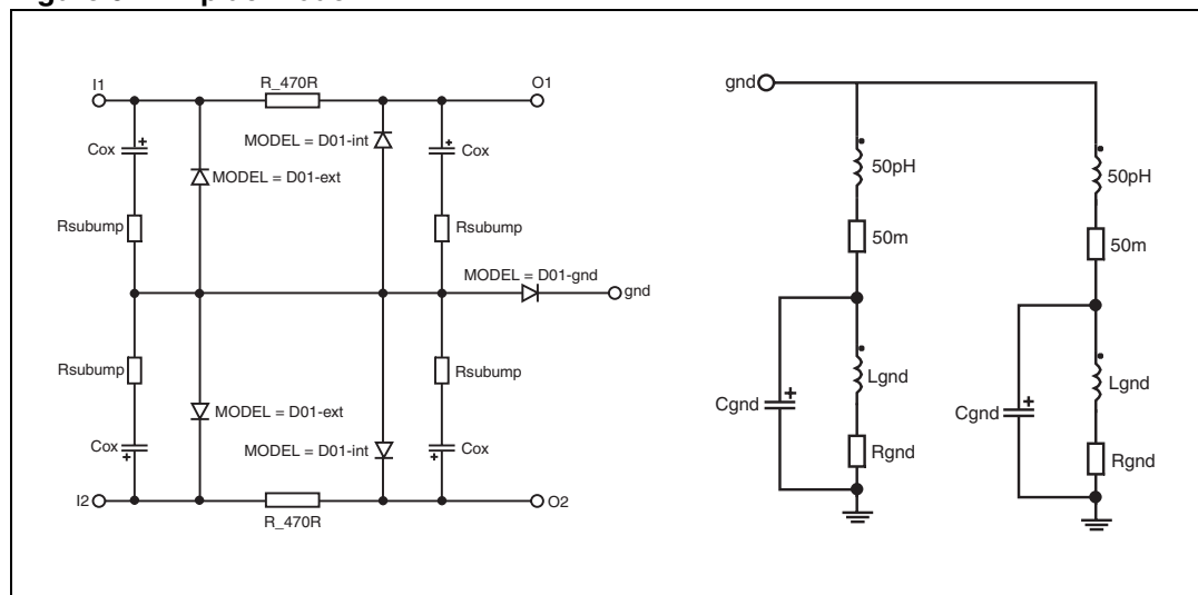
Figure 9. Aplac model
