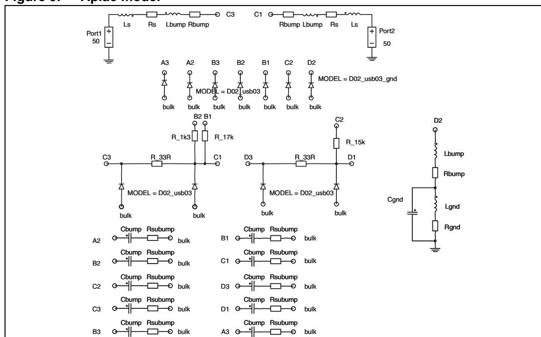
Figure 9. Aplac model
