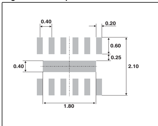
Figure 9. Footprint
