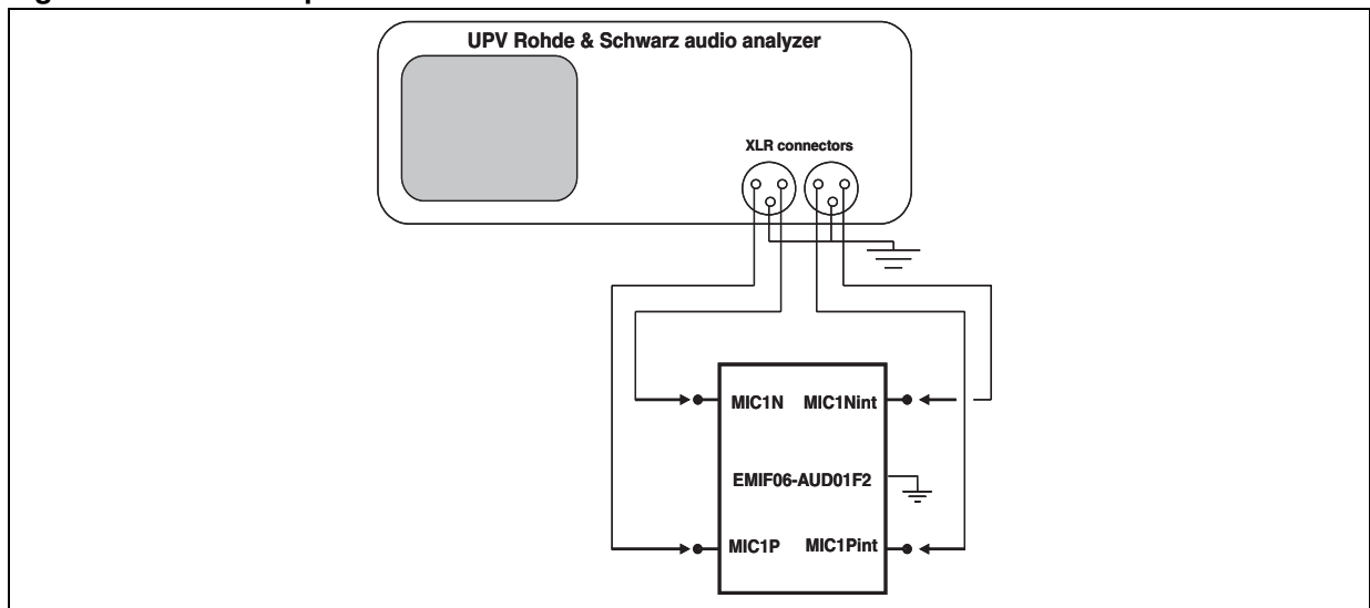
Figure 24. Internal UPV setup schematic
