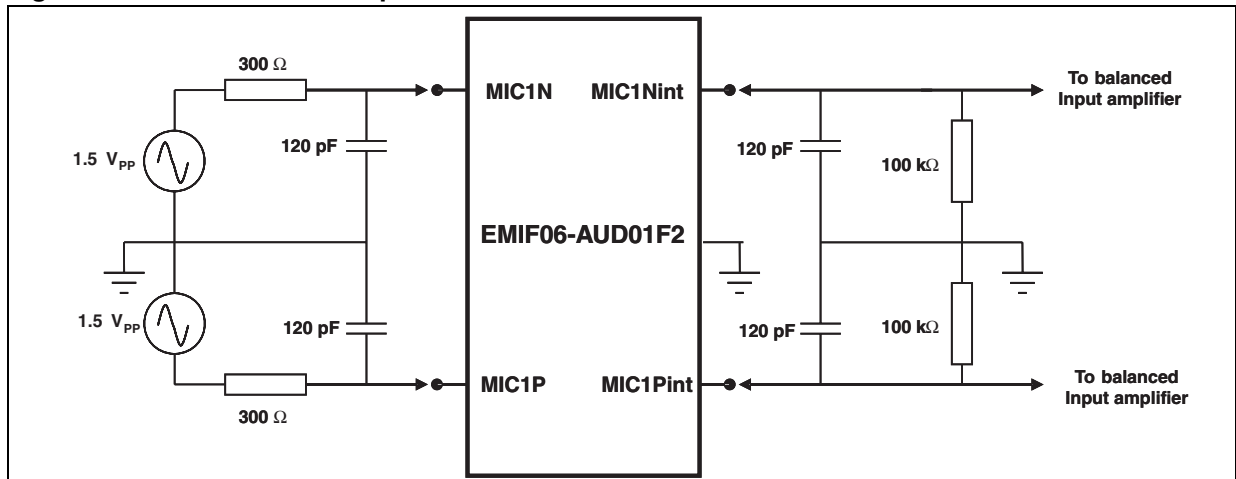
Figure 24. Internal UPV setup schematic
