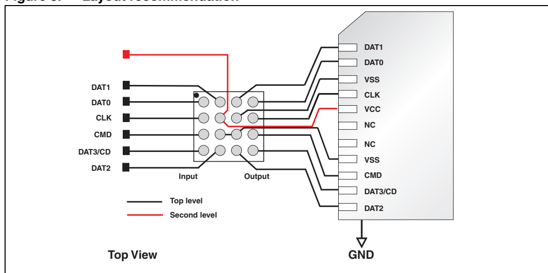
Figure 8. Layout recommendation
