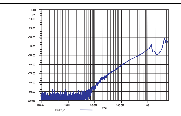
Figure 4. Analog crosstalk
